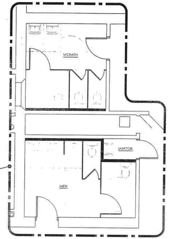
PROPOSED LAYOUT
